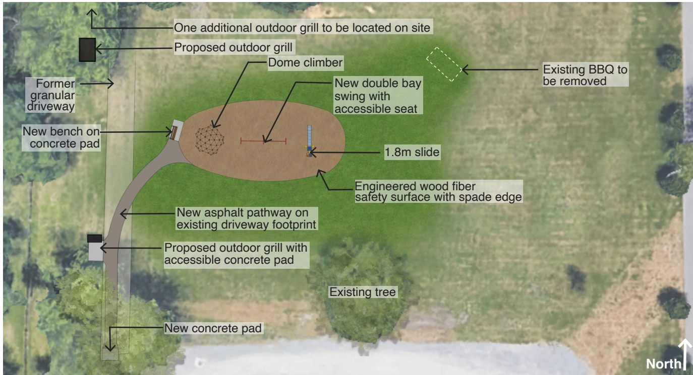
Landscape Plan
