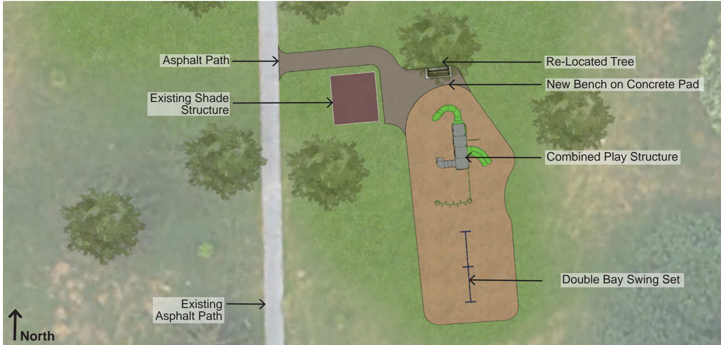
Landscape Plan
